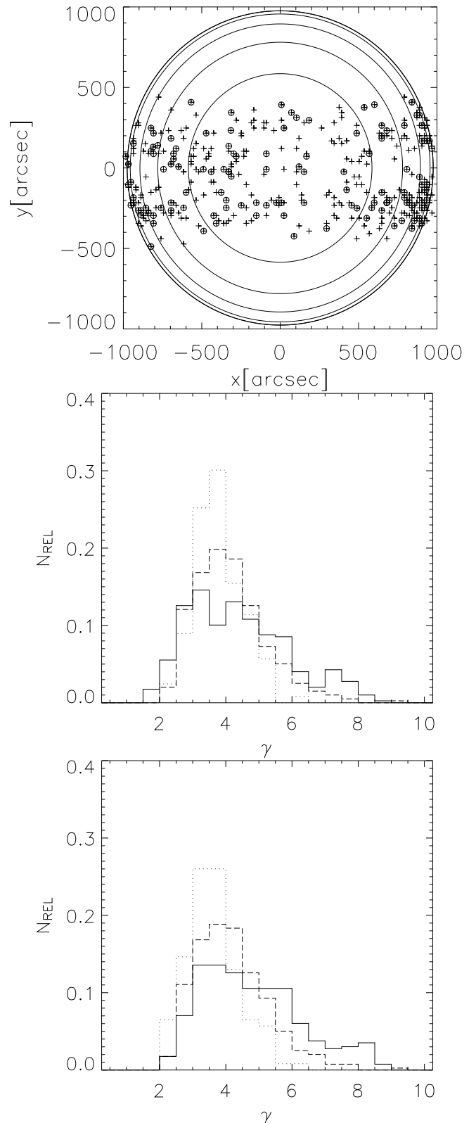
Fig. 3. Top: Positions of selected flares. Crosses indicate 398 flares used for the centre-to-limb analysis of \gamma_0 and \gamma_1 , small circles correspond to 123 flares for the \gamma_2 analysis (see text for details). Large circles indicate regions of \mu = 0.2, 0.4, 0.6, and 0.8 . Middle and bottom: Relative occurrence of \gamma_0 (solid), \gamma_1 (dashed), and \gamma_2 (dotted) from observed spectra and those corrected for isotropic albedo, respectively.
